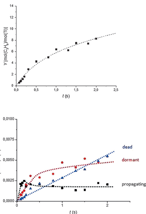
Figure 2. Plots of yield (top) and population distribution of propagating, dormant, and dead (olefin-terminated) chains (bottom) beyond the controlled regime of propene polymerization with \text{MgCl}_2/\text{TiCl}_4/\text{DIBP} and \text{TIBA}/\text{DIBDMSi} at 40 °C. Data from Table 3; the symbols in the bottom plot refer to the chain-end structures in Scheme 2.
